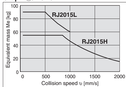
Graph 23/RJ20
