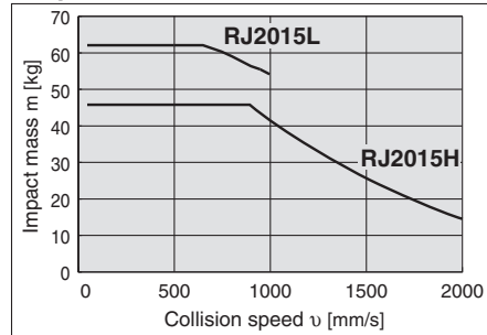
Graph 17/RJ20
