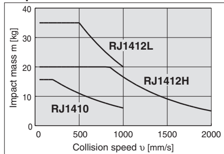
Graph ④/RJ14
