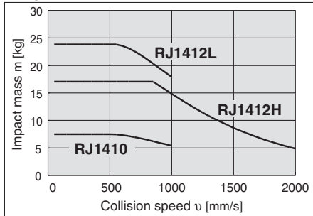
Graph 16/RJ14
