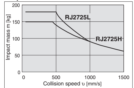
Graph ⑥/RJ27
