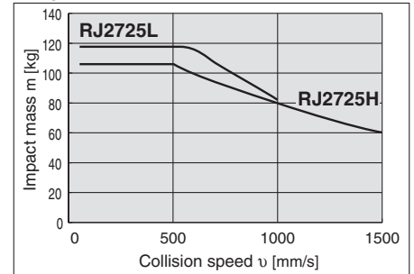
Graph 18/RJ27
