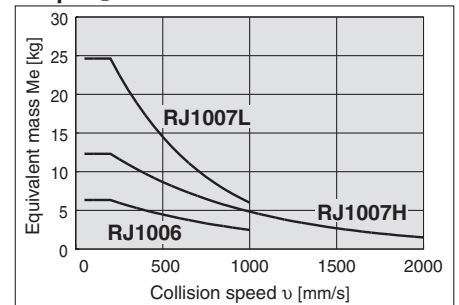
Graph 24/RJ27
