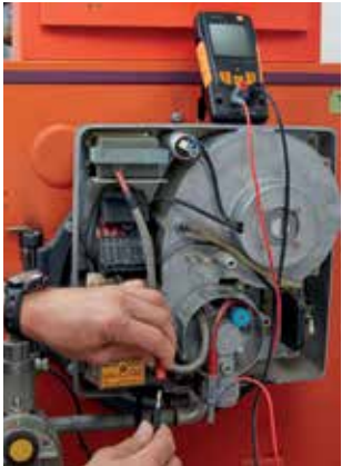
Ionization current measurement set-up
