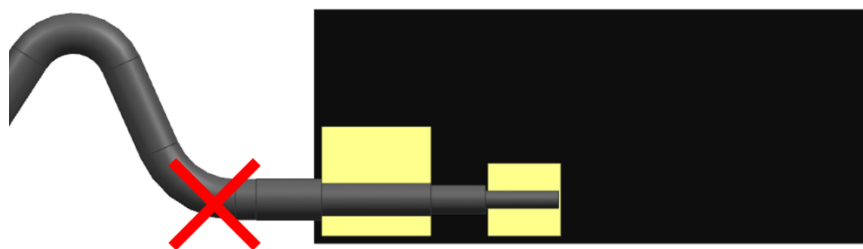
FIGURE 5.2.3 MULTIPLE BENDING OF CABLES IS NOT RECOMMENDED
