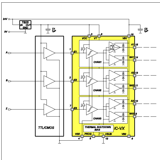
Fig. 3: V_{EE} = V_{SUB}
